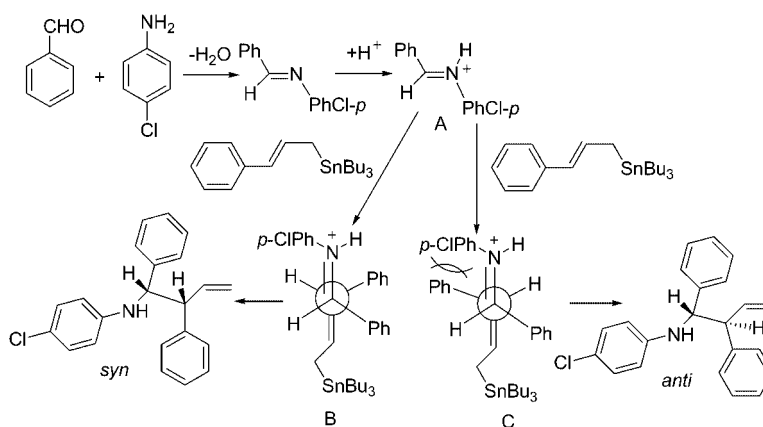
Scheme 1. A plausible mechanism for the Brønsted acid catalyzed imine allylation reaction.
